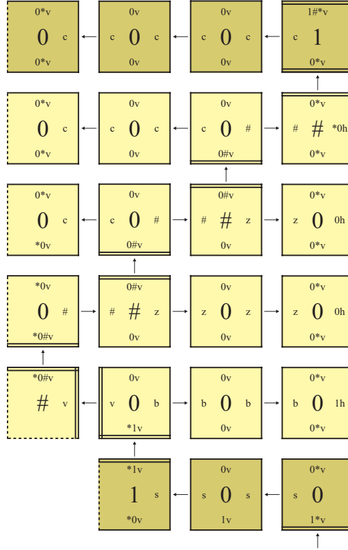
Figure 14: The self-assembly of S_2^\uparrow above the topmost row of \tilde{Y}_1 .
