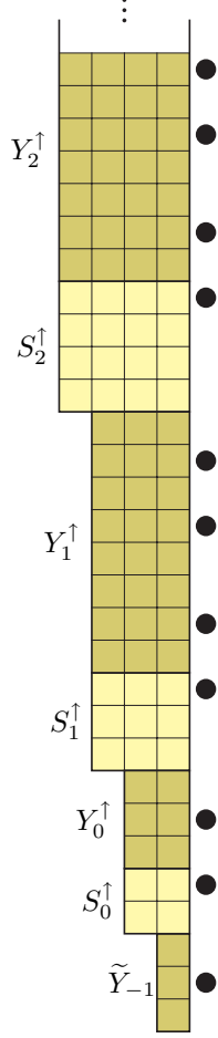
Figure 4: The structure of Y . The dots denote the \theta -points.
