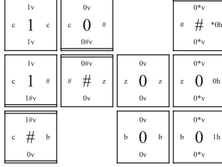
Figure 9: Tile types in which S_n^\uparrow self-assembles.
